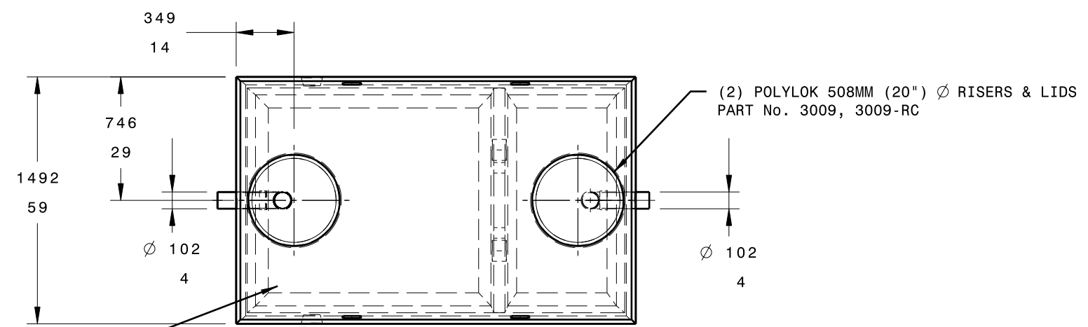
Top view
