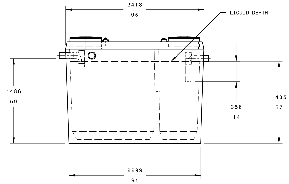
Front view
